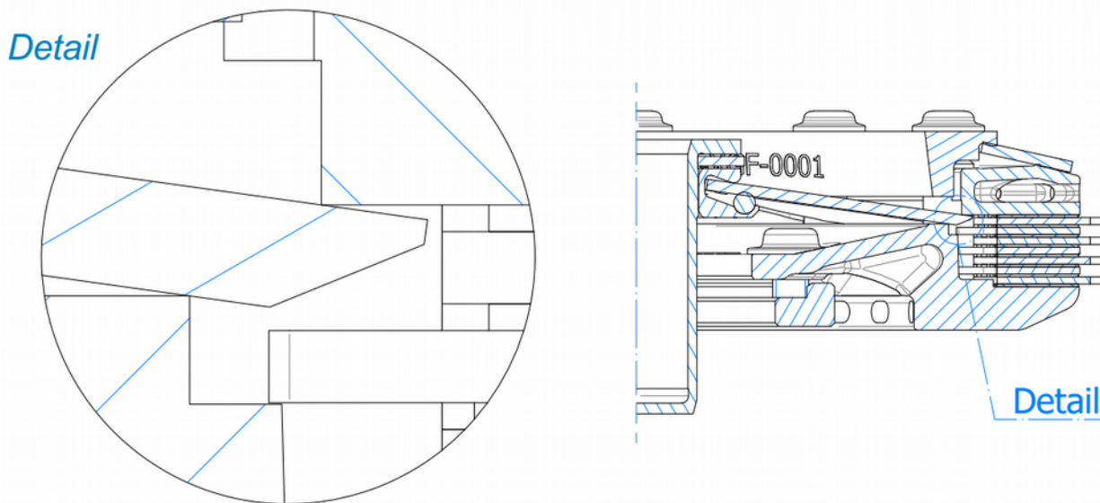
Fig.1. Assembly details
